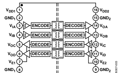
Figure 3. ADuM2402
