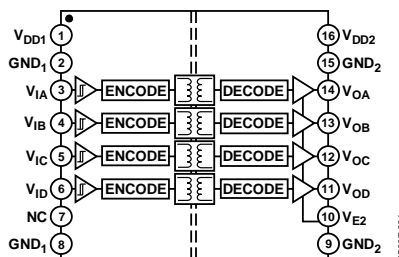
Figure 1. ADuM2400
