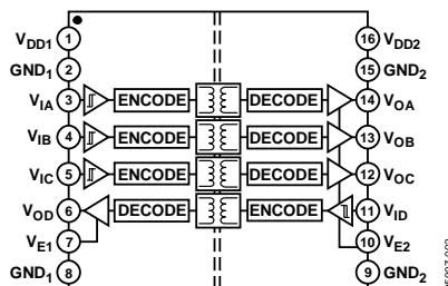
Figure 2. ADuM2401
